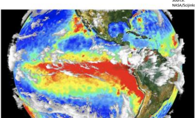
3-D cloud and surface temperature data are combined in this image from the Terra satellite, which shows a well-developed El Niño condition. The red area is warm water sitting off the coast of western South America.
