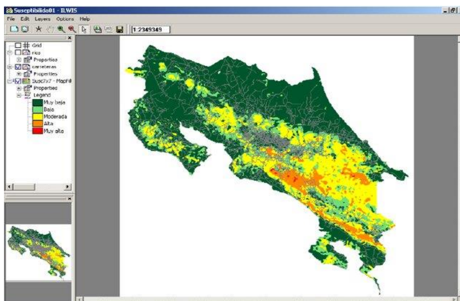
Figure 5. Image of the landslide susceptibility map of Costa Rica – RECLAIMM project. Sourced from ResearchGate.
